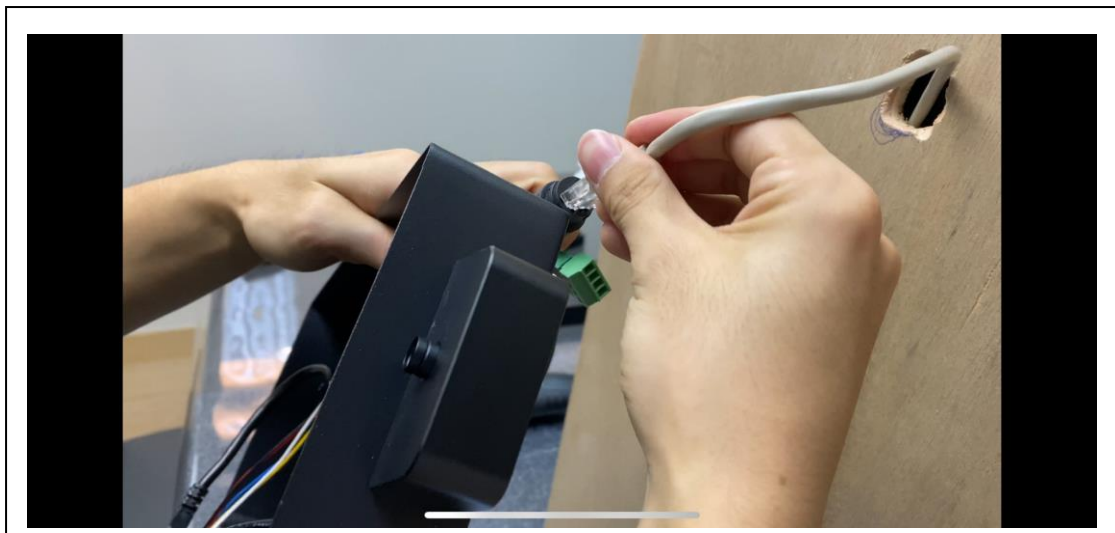
5. Connect PoE from wall to the PoE on metal case.
