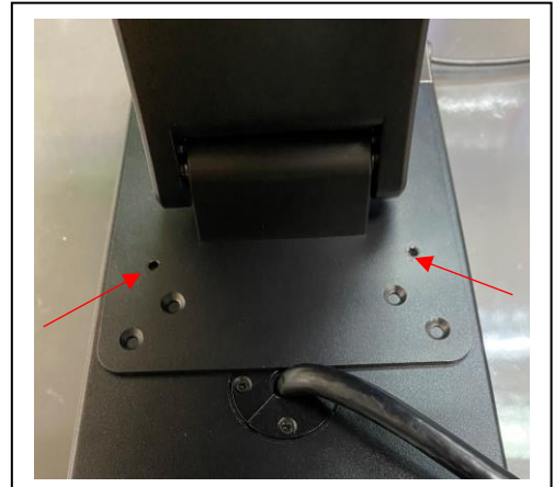
4. Place TAURI7 on table and screw two 3M x 8mm screws here.
