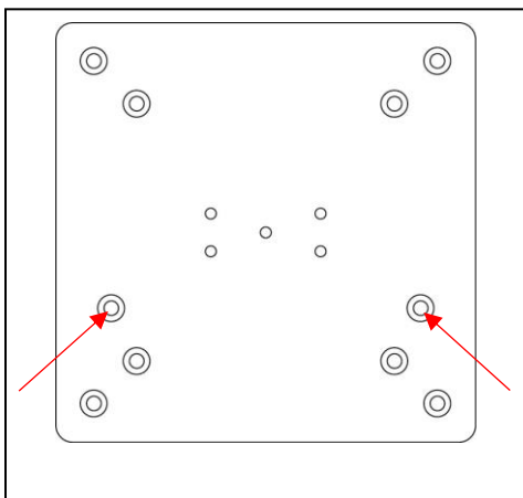
5. The position of the holes in step 4 on metal plate.
