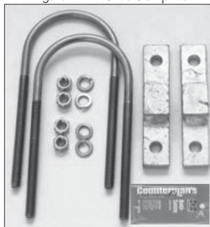
Figure 1: ANTC485 Clamp Kit
