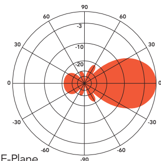
ANT450Y10-WR at 460 MHz
