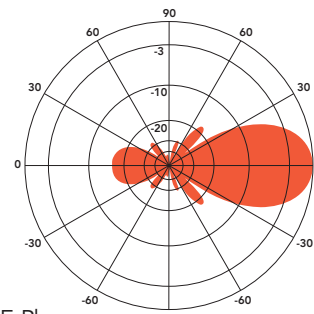
E-Plane Gain: 12.2 dBd
