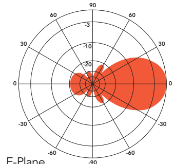
E-Plane Gain: 10.2 dBd
