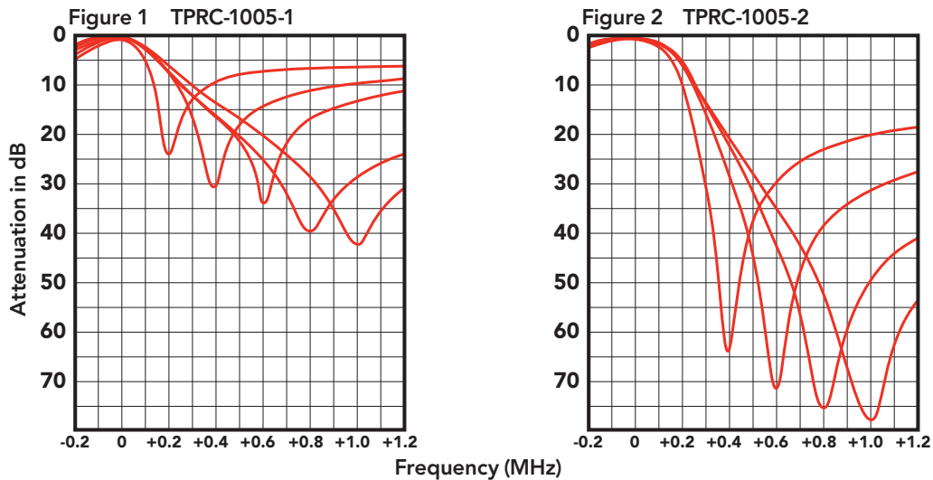
TYPICAL SELECTIVITY CHARACTERISTICS
