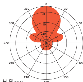
H-Plane Gain: 9.3 dBd
