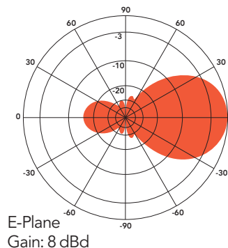
ANT740Y8-WR at 740 MHz
