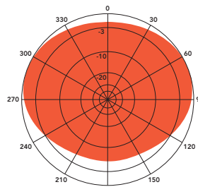
H-Plane gain 8.8 dBd 3/8 wl. spacing from tower
