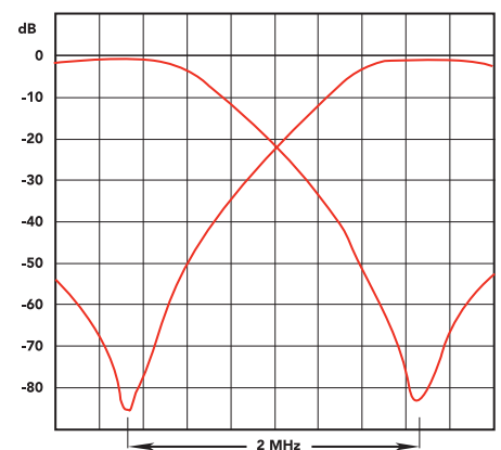
TYPICAL RESPONSE
