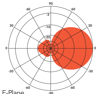
ANT450Y5-WR at 440 MHz
