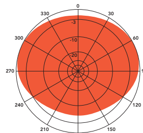
H-Plane gain 9.12 dBd 3/8 wl. spacing from tower
