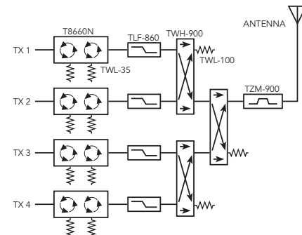
BLOCK DIAGRAM TW860-4HRB1 FOUR CHANNEL HYBRID
