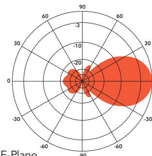
E-Plane Gain: 10.1 dBd
