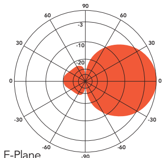
ANT750Y5-WR at 770 MHz
