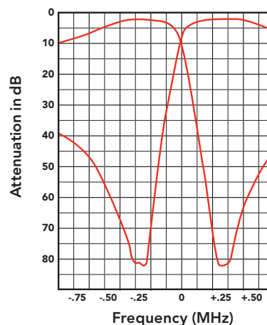
TYPICAL RESPONSE CURVES (TPRD-1484)
