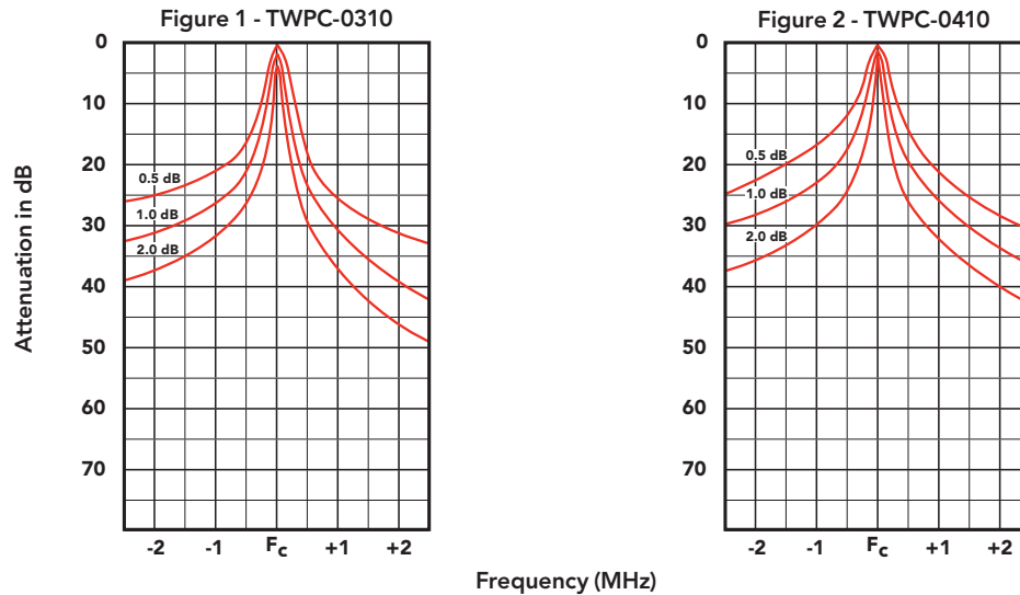
TYPICAL SELECTIVITY CHARACTERISTICS
