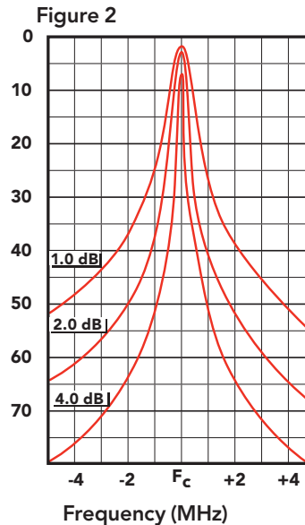
TYPICAL SELECTIVITY CHARACTERISTICS
