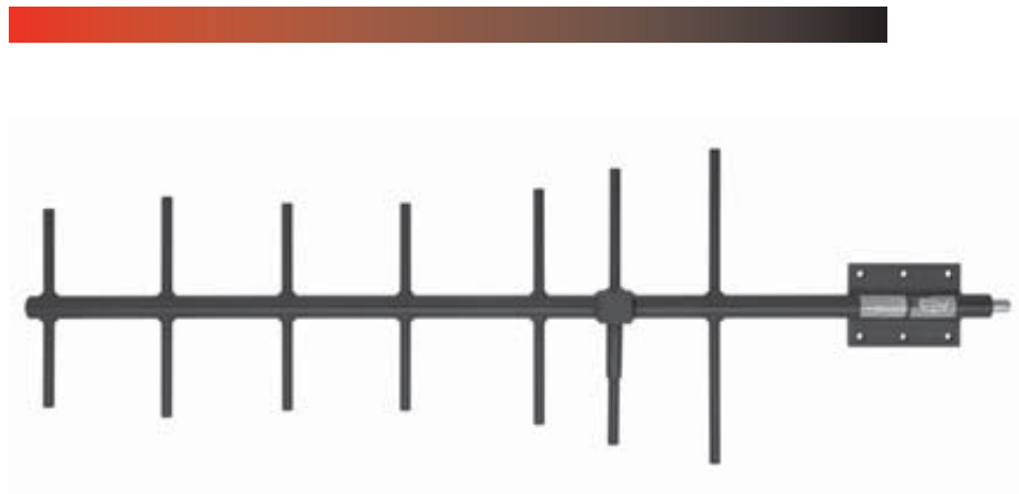
E-Plane Gain: 10.1 dBd
