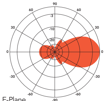
E-Plane Gain: 10.2 dBd
