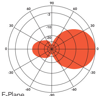
E-Plane Gain: 7.2 dBd
