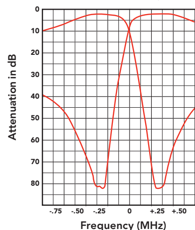
TYPICAL RESPONSE CURVES (TPRD-1084)
