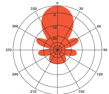
H-Plane Gain: 10.1 dBd
