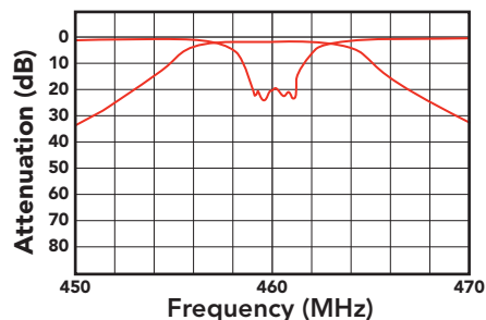
TYPICAL RESPONSE CURVES
