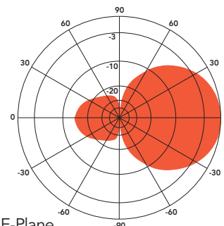
ANT150Y7-WR at 156 MHz
