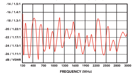
TYPICAL VSWR RESPONSE
