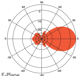
E-Plane Gain: 10.0 dBd
