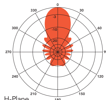
H-Plane Gain: 12.2 dBd
