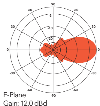
ANT2400Y12-WR at 2450 MHz
