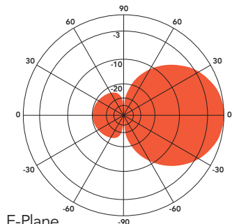
E-Plane Gain: 5.1 dBd
