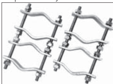
Figure 2: Clamp Preassembly
